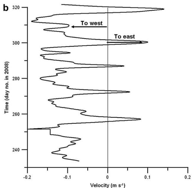
Fig. 6. (a) A time-series plot during the dry season over a tidal cycle of the sea level and dissolved oxygen concentration (D.O.) at mooring site 1 and near surface velocity at mooring site 4. (b) Time-series plot of the low-frequency, longshore velocity near the surface at mooring site 4.
