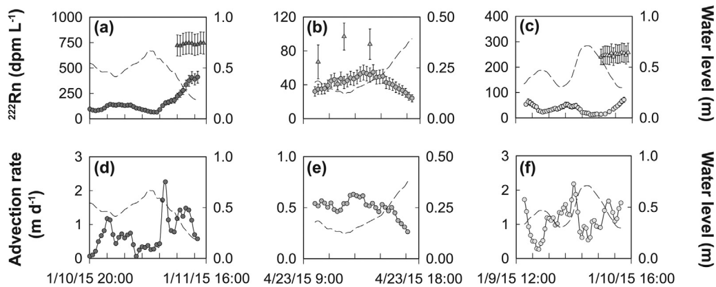
Fig. 2. Time-series ^{222}\text{Rn} in water values for (a) Black Point, (b) Wailupe, and (c) Kawaiui for the coastal sampling station (circular markers) and groundwater samples (triangular markers). Water level is represented by the dashed line. Error bars represent the SD ( 2\sigma ) of ^{222}\text{Rn} measurements. Advection rates (circular markers) are plotted for (d) Black Point, (e) Wailupe, and (f) Kawaiui.
