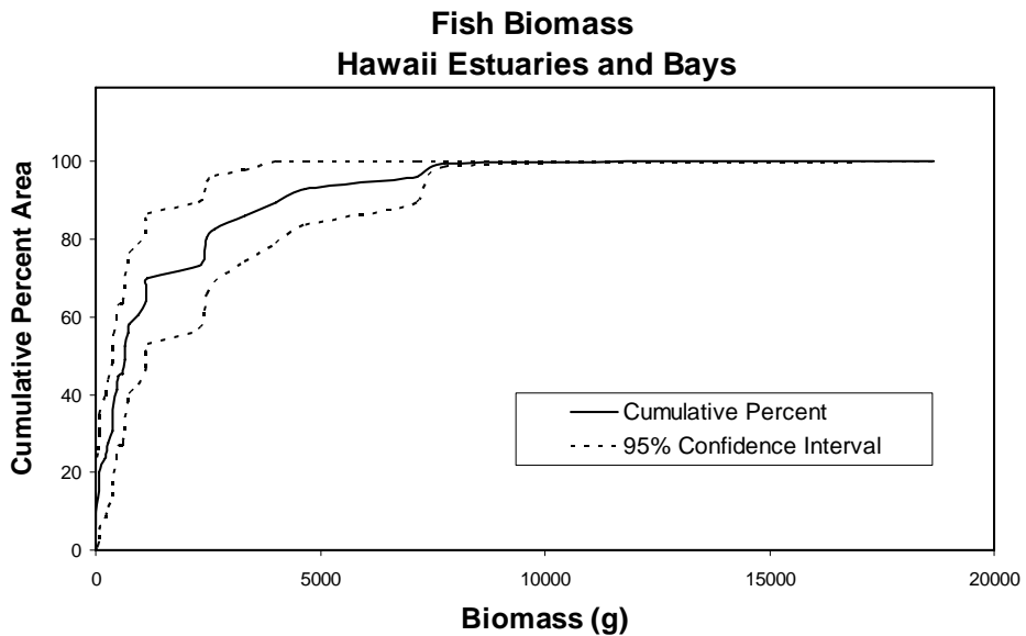
Figure 3.3 -10. Percent area (and 95% C.I.) of Hawaii estuaries and bays vs. the estimated biomass of fishes observed on visual transects.
